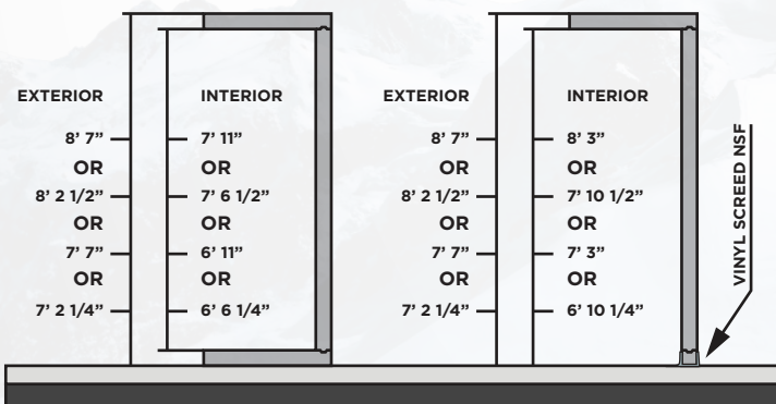
SIDE VIEW WITH FLOOR (RECOMMENDED FOR FREEZERS)
